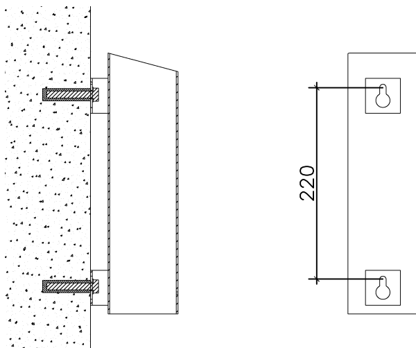
APLICAÇÃO COM 2 BUCHAS METALICA M8 (INCLUIDO) INSTALLATION WITH 2 M8 MECHANIC ANCHORS (INCLUDED)
